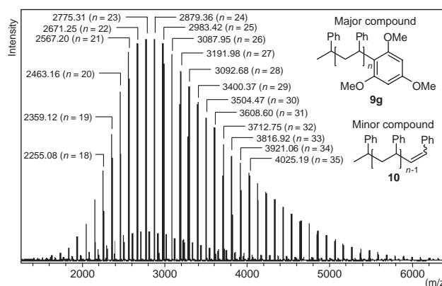
Figure 1. MALDI-TOF mass spectrum of polystyrene 9g and 10 (=93:7). A series of peaks, as indicated by the average mass number, was observed in the silver ion added form ( M + Ag ) + .
